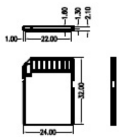
SD CARD
