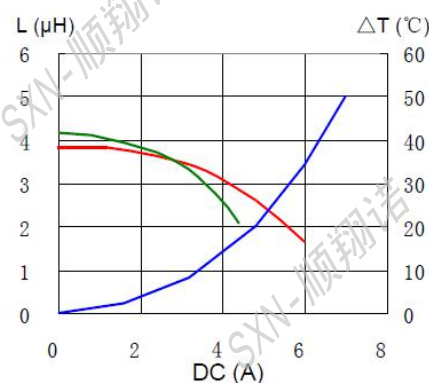
SMRH8D58-3R9N
